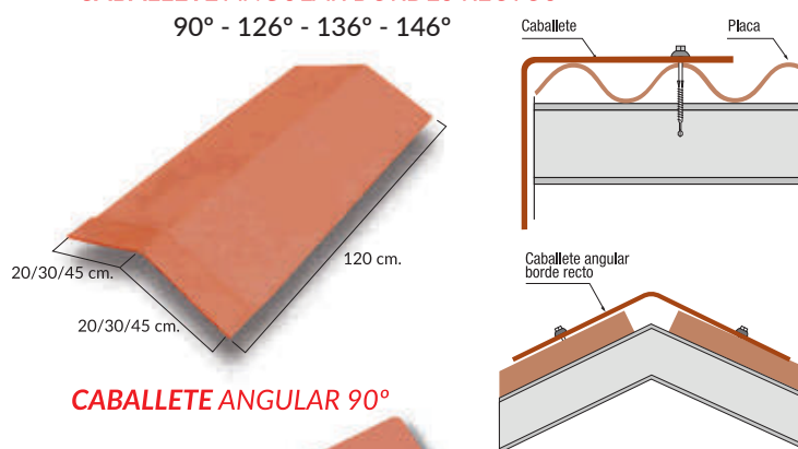
CABALLETE ANGULAR BORDES RECTOS
